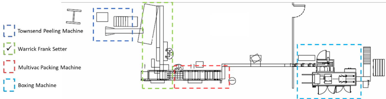
Figure 3. Layout Line 3
