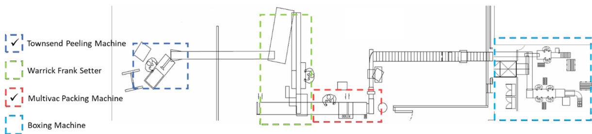
Figure 4. Layout Line 7
