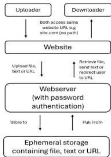
Fig. 1. Web app logic flow diagram
