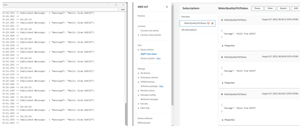
Fig. 11. MQTT Publish test
