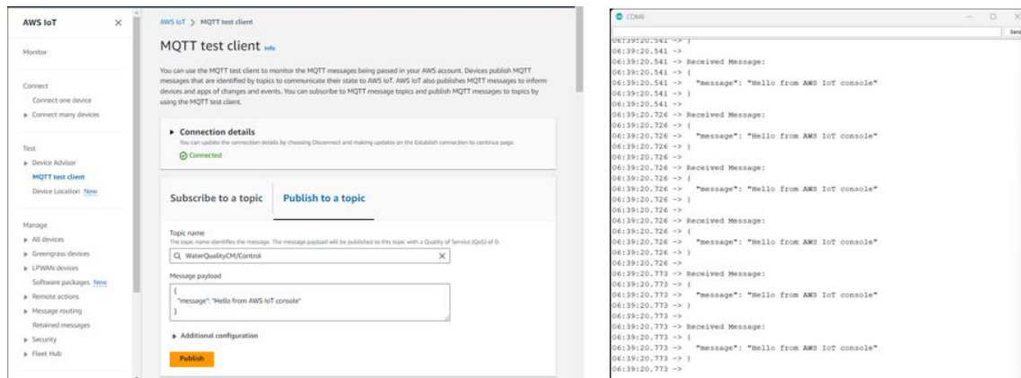
Fig. 12. MQTT Subscribe test
