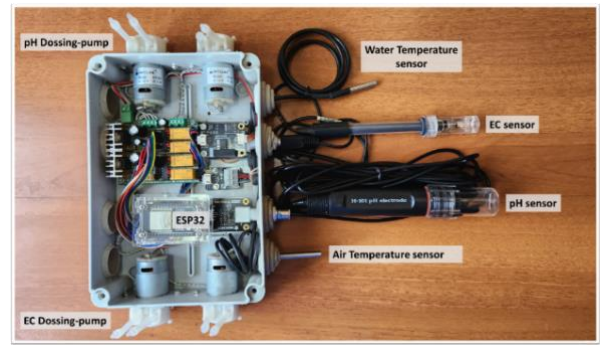
Fig. 3. Hardware of Hydroponic IoT
