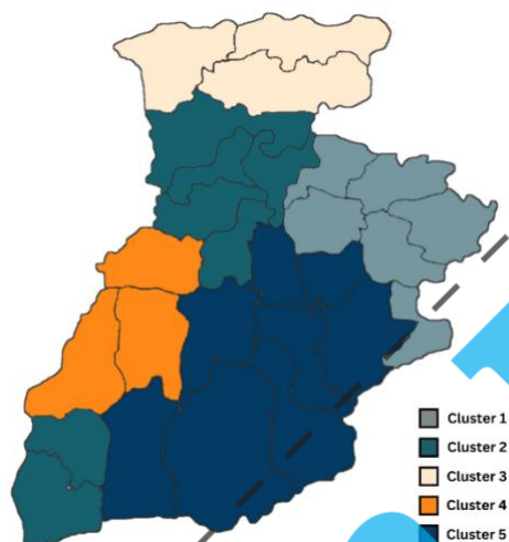
Fig. 10. Spatial Clustering Map with Constraint into K = 5 clusters using the "neighborhood" continuity D1 and the basic infant immunization coverage variables D0 with \alpha = 0.2 .
