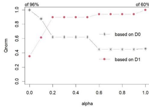
Fig. 9. Proportion of pseudo-inertias that are explained, Q_0^*(P_K^\alpha) versus \alpha (black solid line) and Q_1^*(P_K^\alpha) versus \alpha (dashed line)
