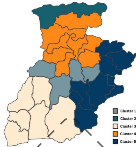
Fig. 7. Spatial Clustering Map with Constraint into K=5 clusters according to the "neighborhood" distances of the districts D1 with \alpha = 0.4 and basic infant immunization coverage D0.
