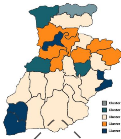
Fig. 3. Spatial Clustering Map without Constraint
