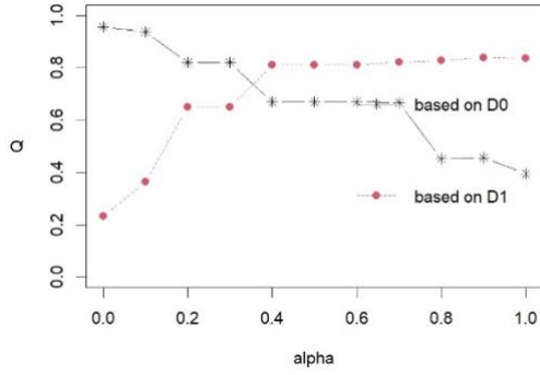
Fig. 5. Proportion of pseudo-inertias that are explained, Q_0(P_K^\alpha) versus \alpha (shown as a black solid line) and Q_1(P_K^\alpha) versus \alpha (shown as a dashed line).
