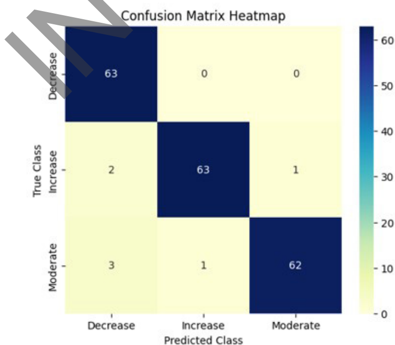
Figure 6. Confusion Matrix
