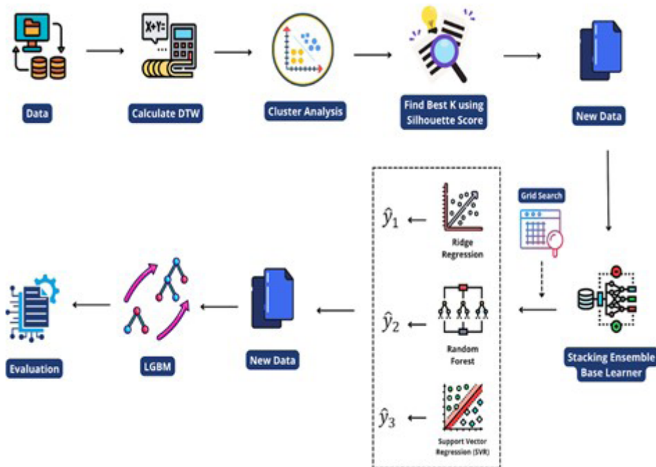
Figure 2 Proposed Method: STACKEL K-MEANS
