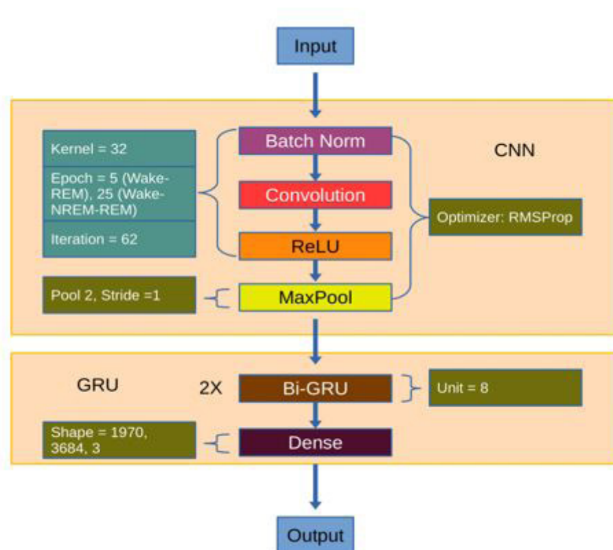
Figure 2 CNN-GRU Model
