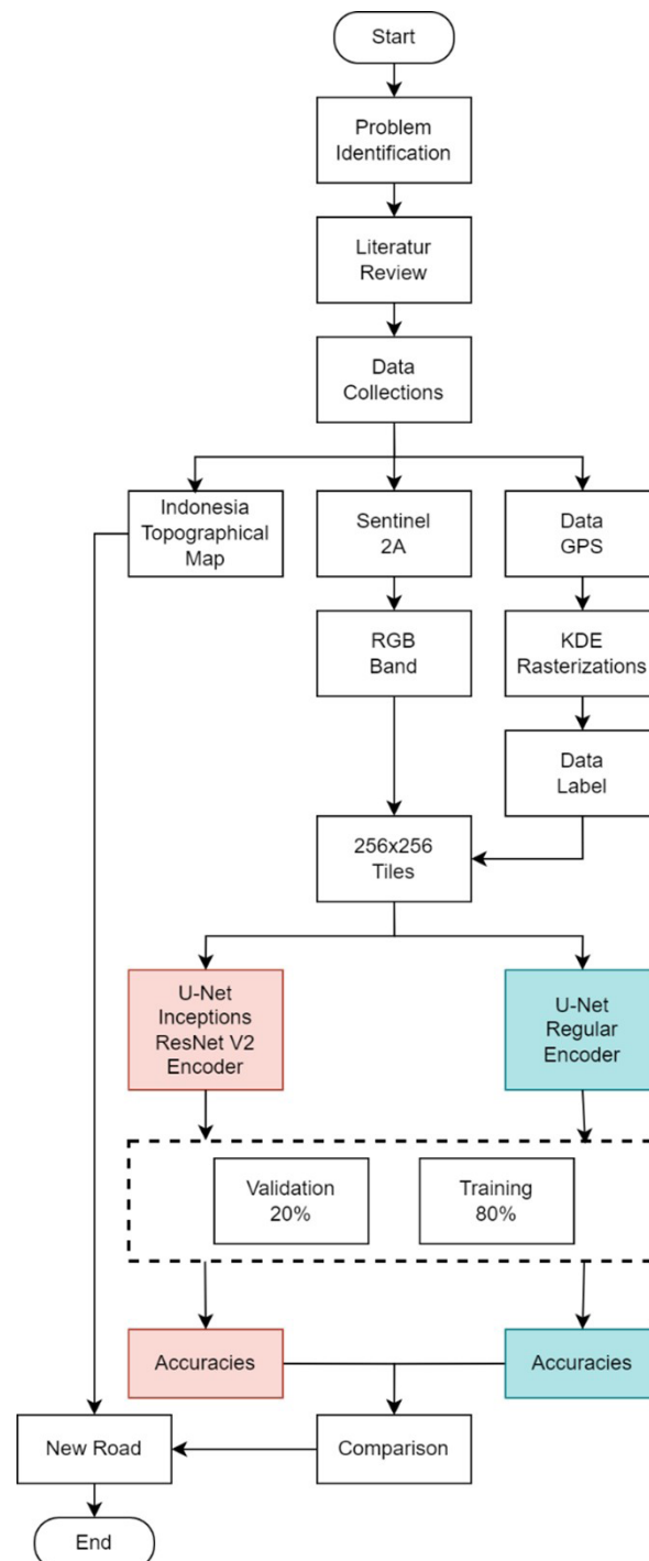
Figure 1 Research Flow
