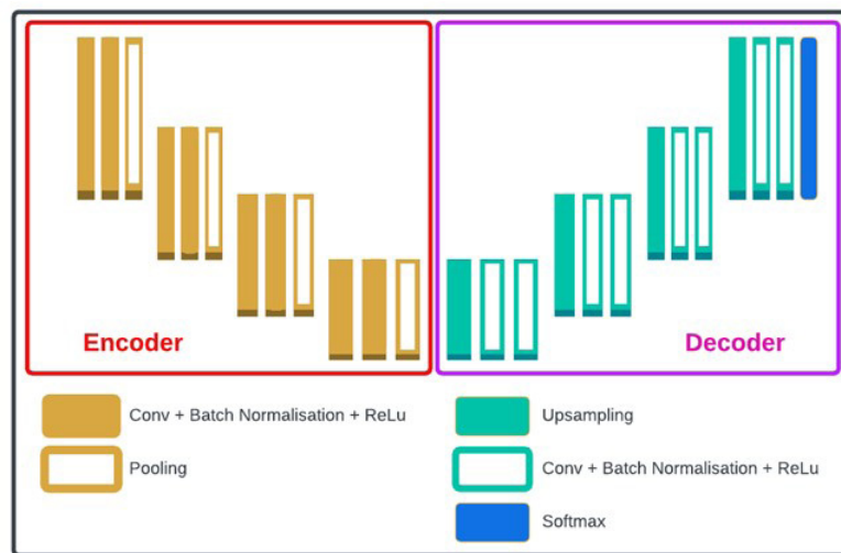
Figure 6 U-Net Architecture
