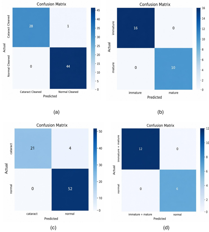
Fig. 6. Confusion matrix of Dataset 1–4 after cleaning.
