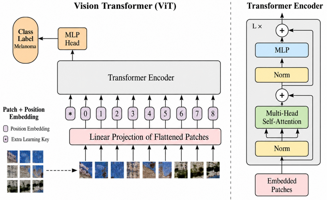
Fig. 3. Vision Transformer (ViT) illustration by Dosovitskiy et al. [22]. Note: Multi-Layer Perceptron (MLP).
