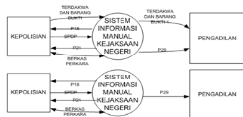
Fig. 7 Diagram of data flow for the current (top) and future architecture (below)
