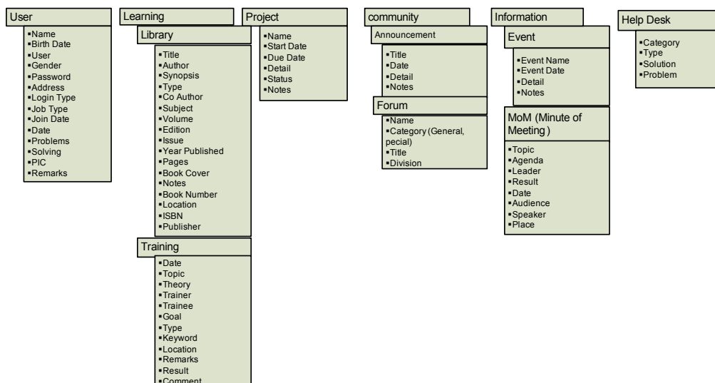
Figure 3 Menu Structure
