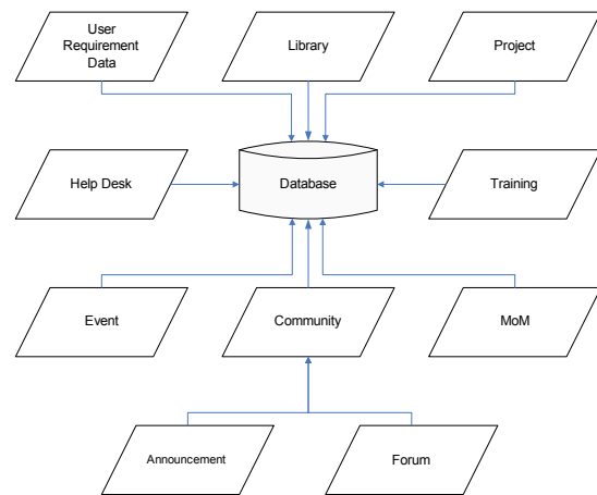
Figure 2 Database Framework
