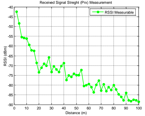
Fig. 8. The result of P_{RX} measurement.
