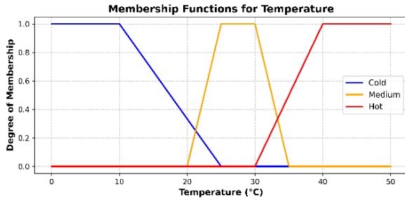
Fig. 5. Temperature membership function.
