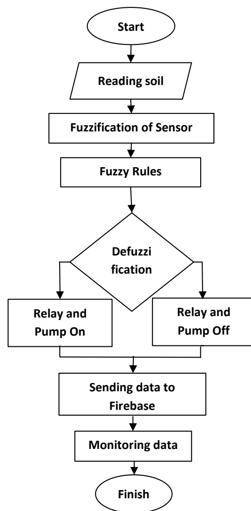
Fig. 3. Flowchart of IoT-based drip irrigation system for tobacco crops.
