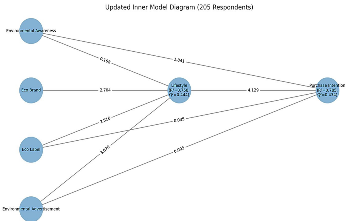
Figure 1 Results of Inner Model
