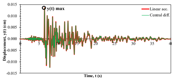
Figure 3. Comparison of relative SDof displacement time histories calculated using the linear acceleration and central difference methods at T = 0.04 s and 5% damping.
