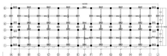
Figure 4. Plan view of the reinforced concrete beam layout used in the five-story building model; beam sizes and BI/BA codes are listed in Table 4.
