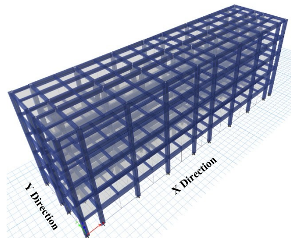
Figure 5. Three-dimensional ETABS model of the five-story reinforced concrete special moment-resisting frame, showing the X and Y principal directions and the 4.2 m story height.
