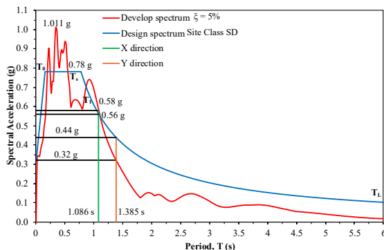
Figure 9. Comparison of 5%-damped pseudo spectral acceleration (PSA, g) for the developed Yogyakarta event-based spectrum and SNI 1726:2019 design spectrum (Site Class SD), with the X- and Y-direction fundamental periods marked.
