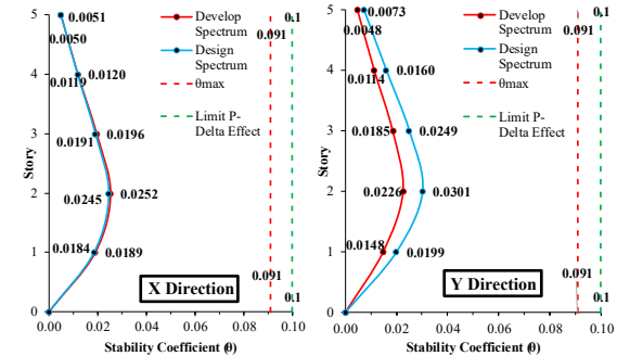
Figure 17. P-Delta stability coefficients (dimensionless) in the X and Y directions for the developed and SNI 1726:2019 design response spectra, calculated with force-scaled story shears and Cd/Ie-amplified design drifts; dashed lines show \theta_{max} = 0.091 and \theta = 0.10 .
