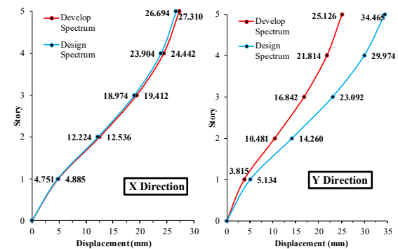
Figure 15. Unscaled elastic floor displacement profiles (mm) in the X and Y directions from the developed and SNI 1726:2019 design response spectra, before Cd/Ie amplification.
