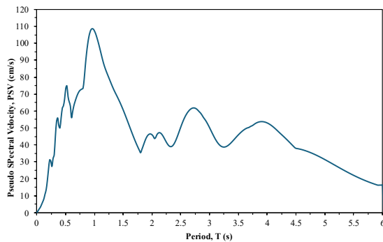
Figure 8. Pseudo spectral velocity (PSV, cm/s) calculated from the synthetic Yogyakarta earthquake acceleration time history at 5% damping.
