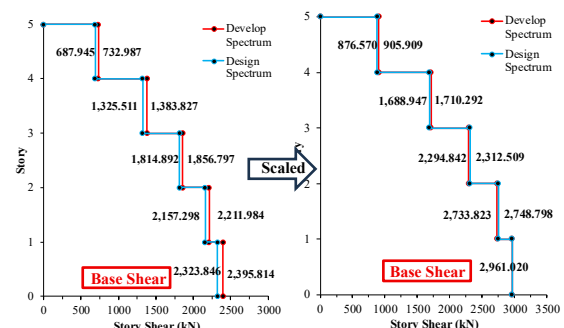
Figure 13. X-direction story shear distributions (kN) from the developed and SNI 1726:2019 design response spectra before and after force scaling
