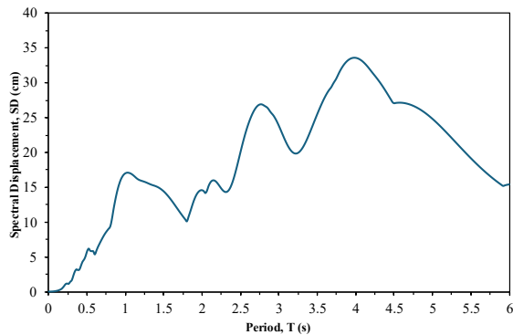
Figure 7. Spectral displacement (SD, cm) calculated from the synthetic Yogyakarta earthquake acceleration time history using the linear acceleration method at 5% damping.
