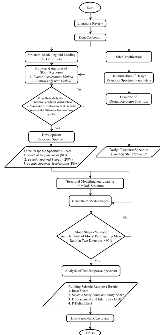
Figure 1. Computational workflow for developing the 5%-damped response spectrum from the synthetic 2006 Yogyakarta earthquake time history and comparing building responses with SNI 1726:2019.
