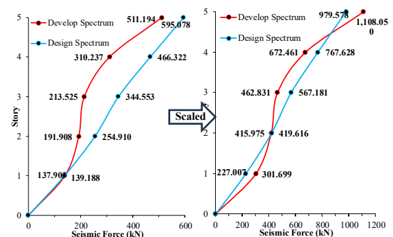
Figure 12. Y-direction seismic story force distributions (kN) from the developed and SNI 1726:2019 design response spectra before and after force scaling
