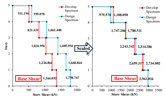
Figure 14. Y-direction story shear distributions (kN) from the developed and SNI 1726:2019 design response spectra before and after force scaling.
