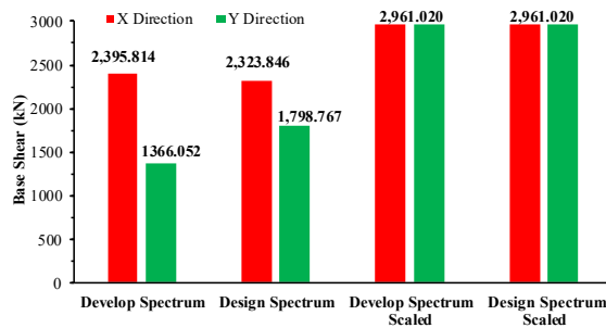
Figure 10. Unscaled and force-scaled seismic base shear (kN) in the X and Y directions for the developed and SNI 1726:2019 design response spectra.
