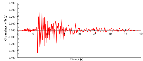
Figure 2. Synthetic 2006 Yogyakarta earthquake acceleration time history attributed to Pawirodikromo, (2014), with a 40 s duration, 0.01 s time step, and peak ground acceleration of 0.3373 g.
