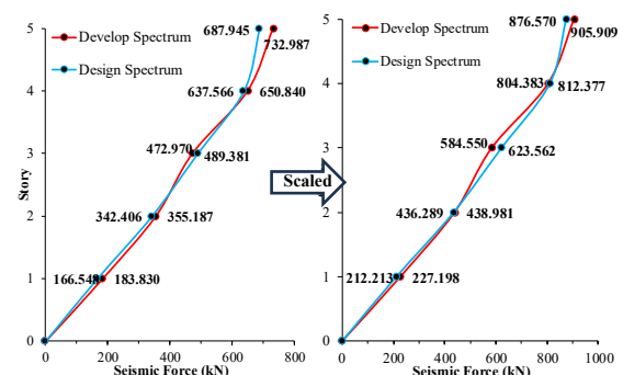
Figure 11. X-direction seismic story force distributions (kN) from the developed and SNI 1726:2019 design response spectra before and after force scaling.
