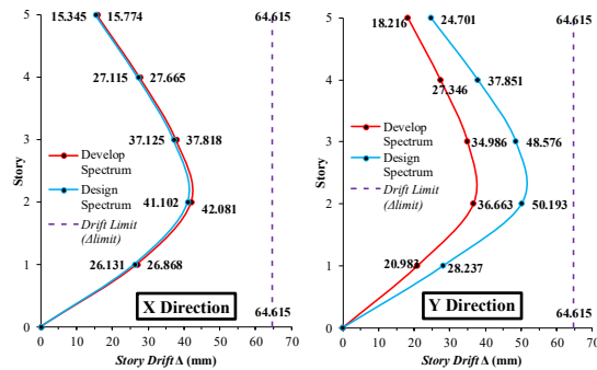
Figure 16. Design inter-story drift distributions (mm) in the X and Y directions from the developed and SNI 1726:2019 design response spectra, calculated using Cd/Ie-amplified displacements; dashed lines indicate the adopted 64.615 mm drift limit.
