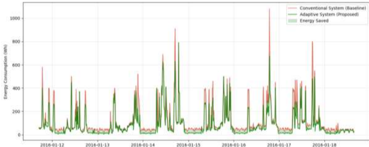
Figure 2. Comparison Baseline vs Adaptive Control
