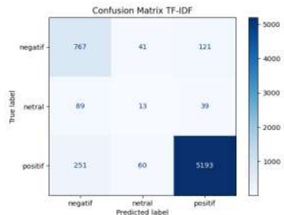
Figure 3. TF-IDF Confusion Matrix Results
