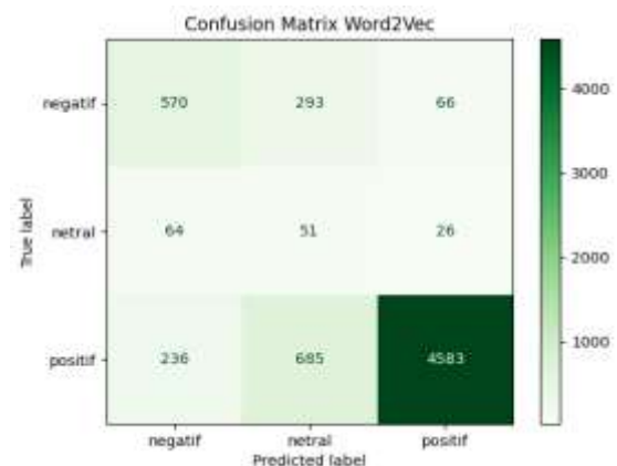
Figure 4. Word2Vec Confusion Matrix Results
