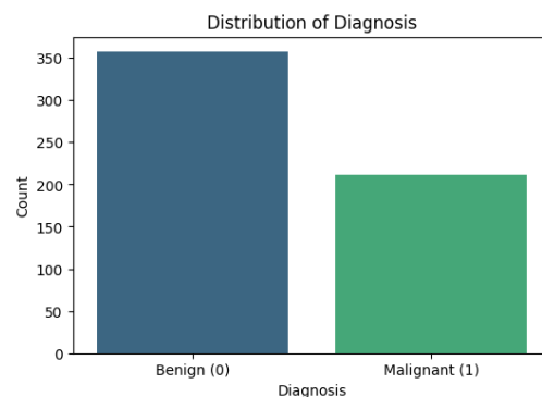
Figure 1. Data Distribution
