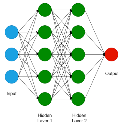
Figure 3. MLP Architecture
