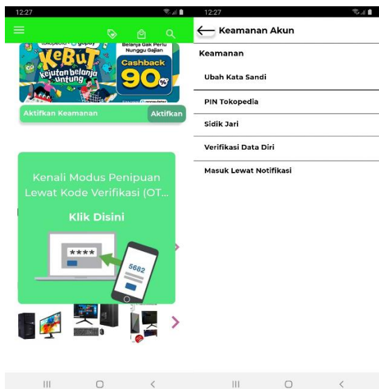
Figure 2. Notification Features
