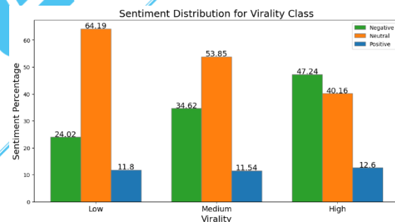
Figure 3 Sentiment Distribution
