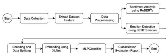
Figure 2. Proposed Methodology
