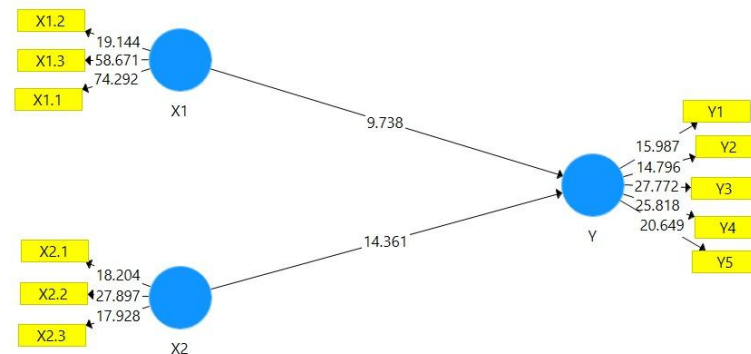
Figure 2. Bootstrapping
